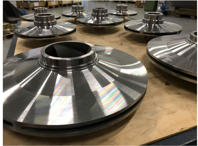
Figure 5 ETL Impeller
